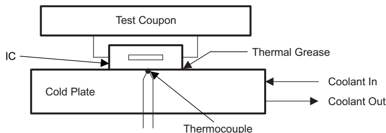
Figure 4. Cu Cold Plate Measurement Process
